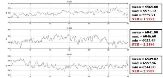
Chaos-Based Applications
