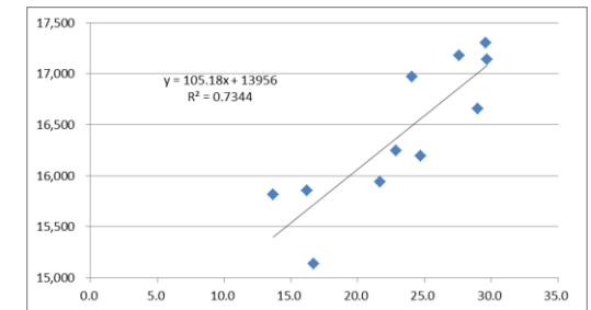
建築能耗基準線圖 Building energy baseline figure
